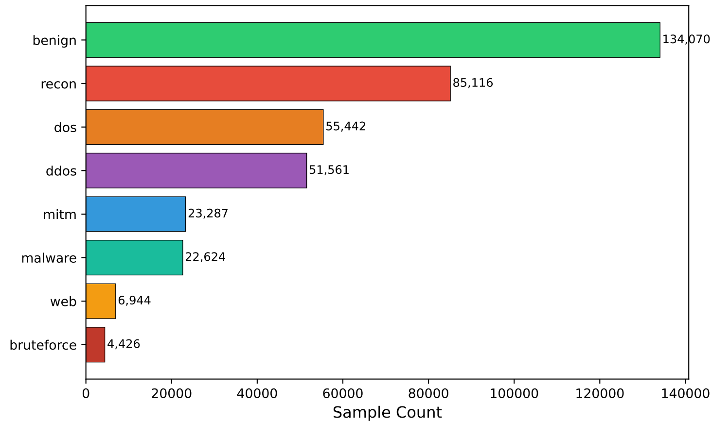
CIC IoT 2025 — Consolidated Class Distribution
